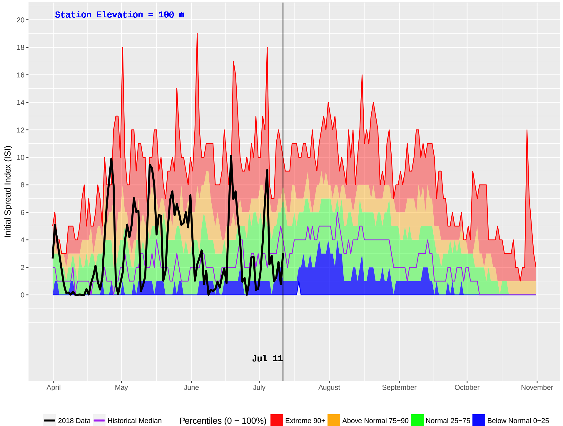
BEAVER CREEK (37) : Historical (1987–2016) and Current (2018) Noon Initial Spread Index (ISI)
